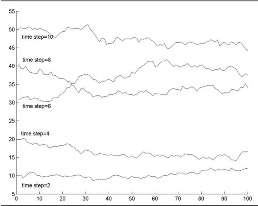
EXHIBIT 8.2 Illustration of the Fractal Properties of the Paths of a Brownian Motion a
